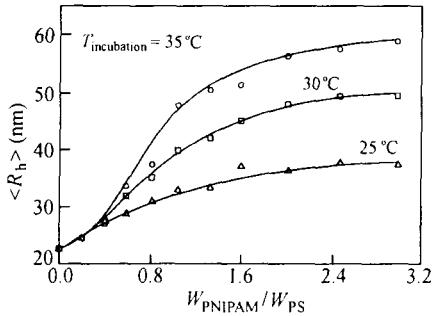
Fig. 1 Incubation temperature ( T_{\text{incubation}} ) and relative polymer concentration ( W_{\text{PNIPAM}}/W_{\text{PS}} ) dependence of the average hydrodynamic radius ( \langle R_h \rangle ) of surfactant-free polystyrene (PS) nanoparticles adsorbed with PNIPAM
