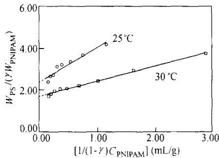
Fig. 6 Adsorption isotherms at two temperatures
